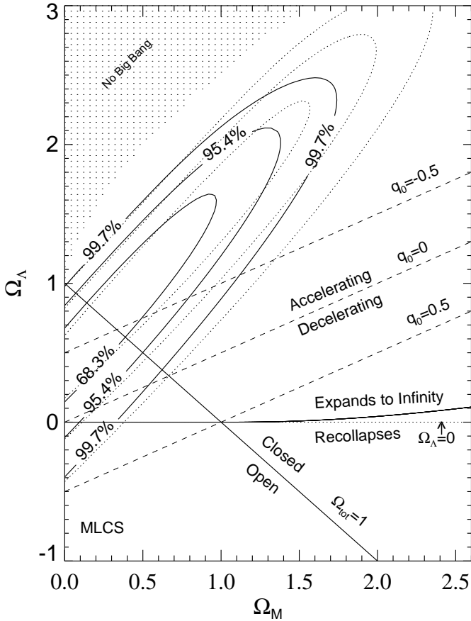
FIG. 6.—Joint confidence intervals for (\Omega_M, \Omega_\Lambda) from SNe Ia. The solid contours are results from the MLCS method applied to well-observed SNe Ia light curves together with the snapshot method (Riess et al. 1998b) applied to incomplete SNe Ia light curves. The dotted contours are for the same objects excluding the unclassified SN 1997ck ( z = 0.97 ). Regions representing specific cosmological scenarios are illustrated. Contours are closed by their intersection with the line \Omega_M = 0 .
